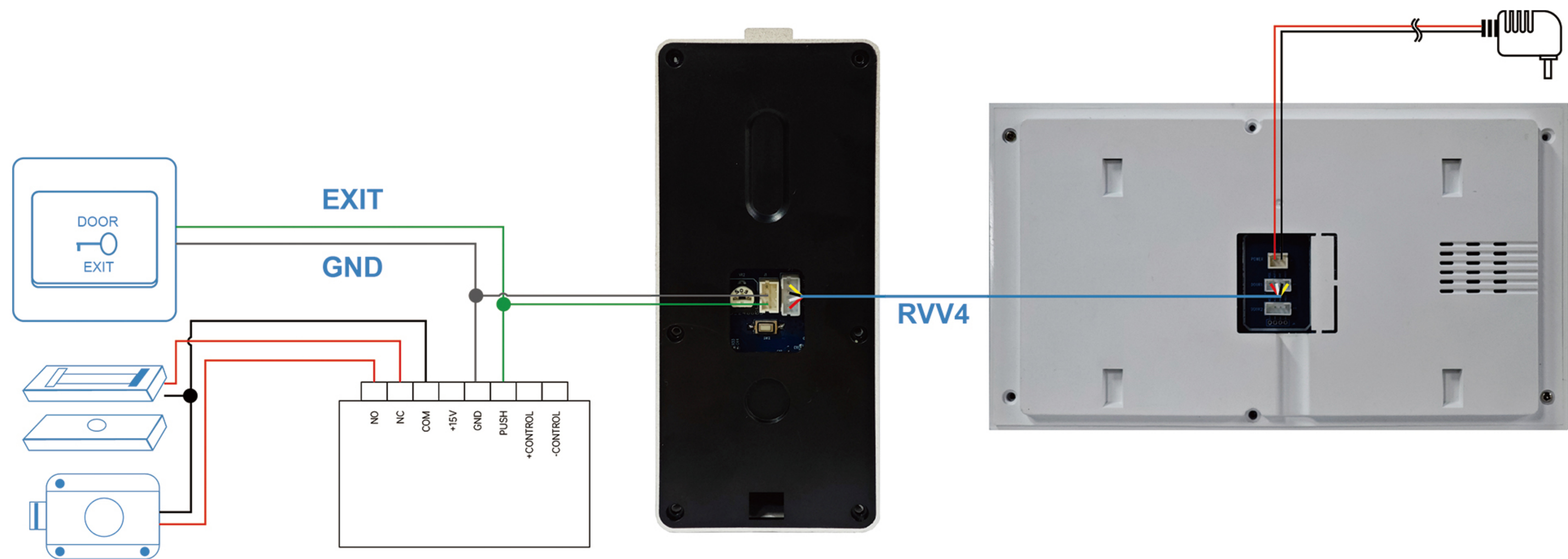
1 Set Outdoor Station to 1 Set Indoor Monitor
