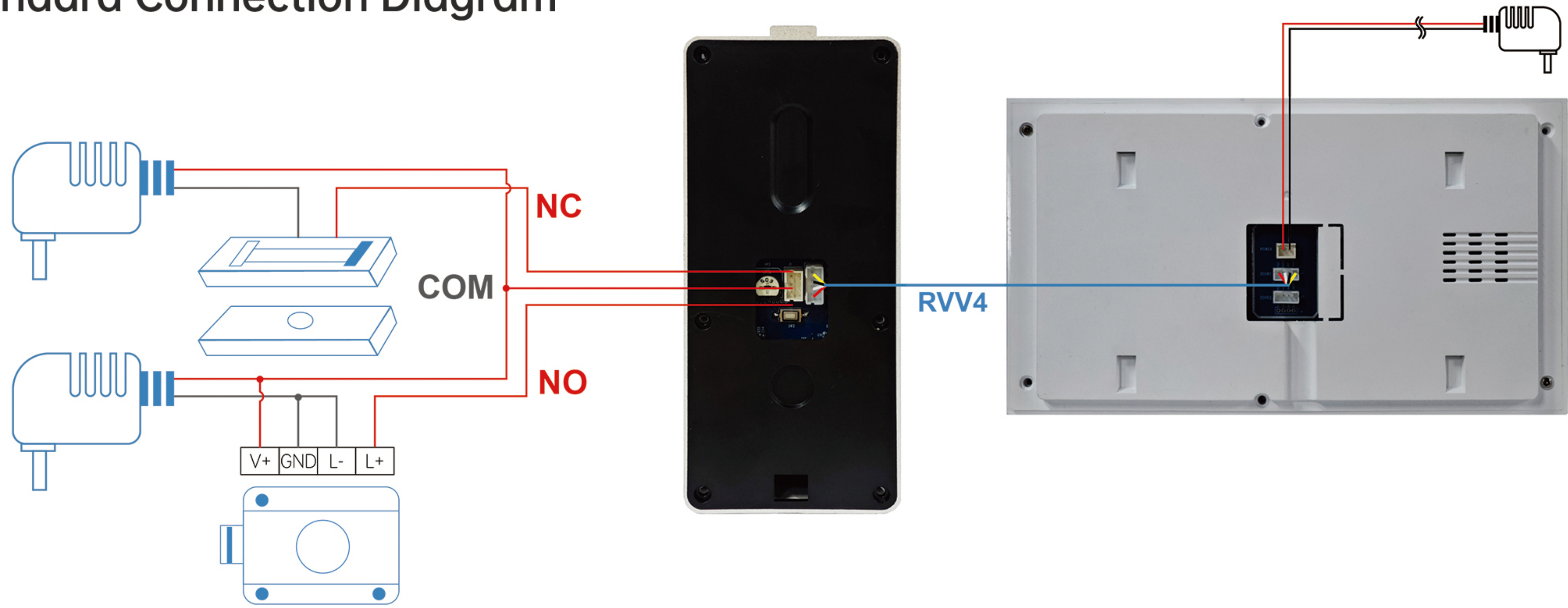
1 Set Outdoor Station to 1 Set Indoor Monitor
